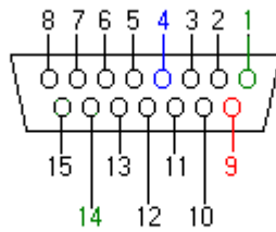
DB-15M CONNECTOR (SOLDER SIDE VIEW)
